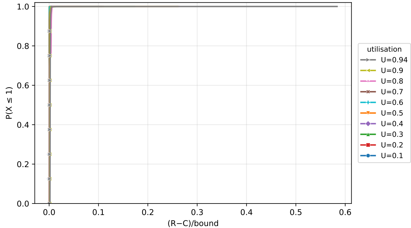
CDF of normalized \Delta (soft)
