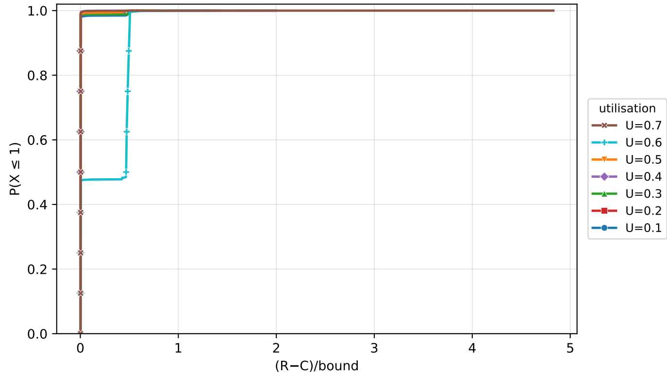
CDF of normalized \Delta (tight)
