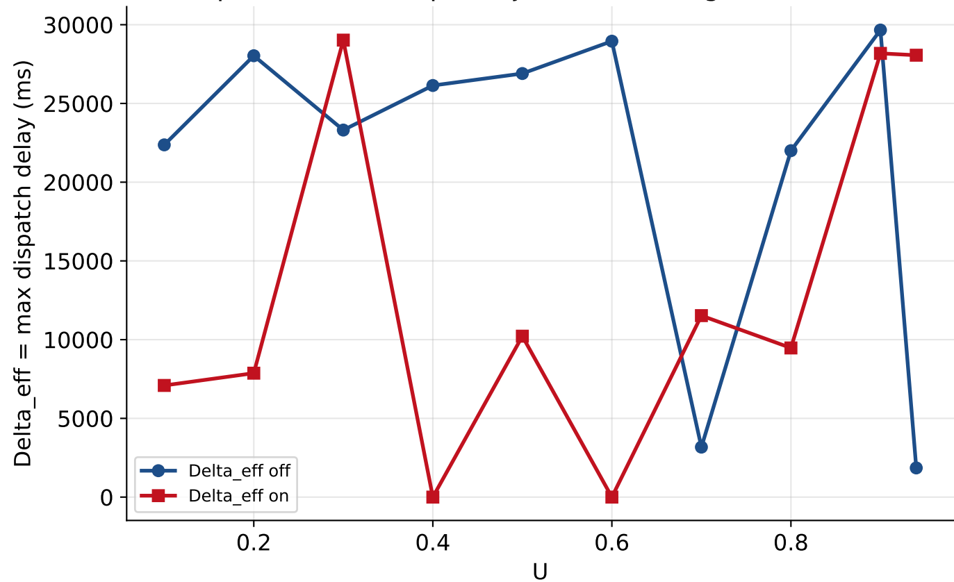
Replenishment/dispatch jitter vs U — tight (P=10 ms)
