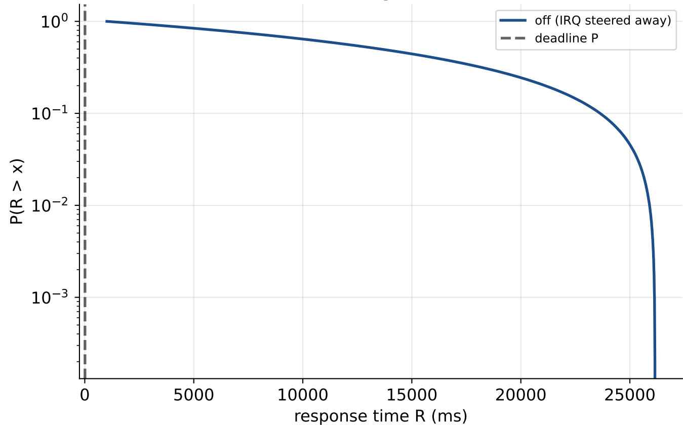
R CCDF off vs on — tight (P=10 ms) U=0.4
