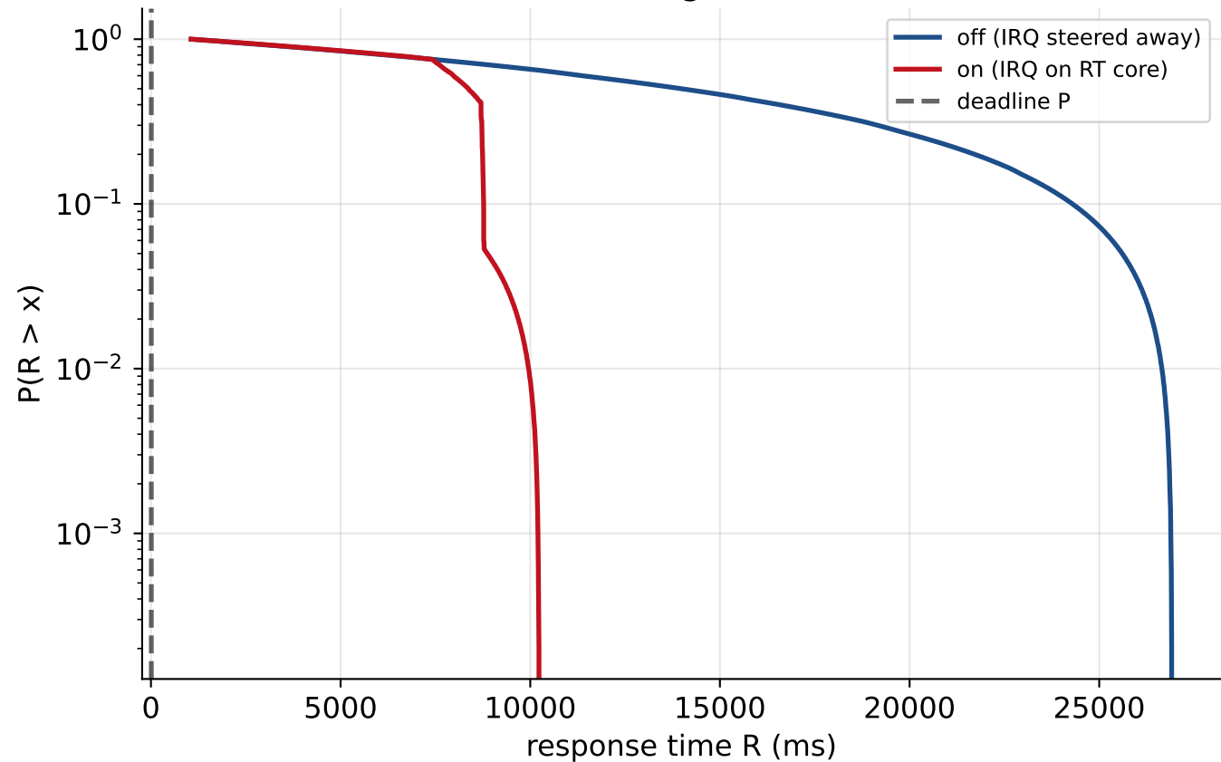
R CCDF off vs on — tight (P=10 ms) U=0.5
