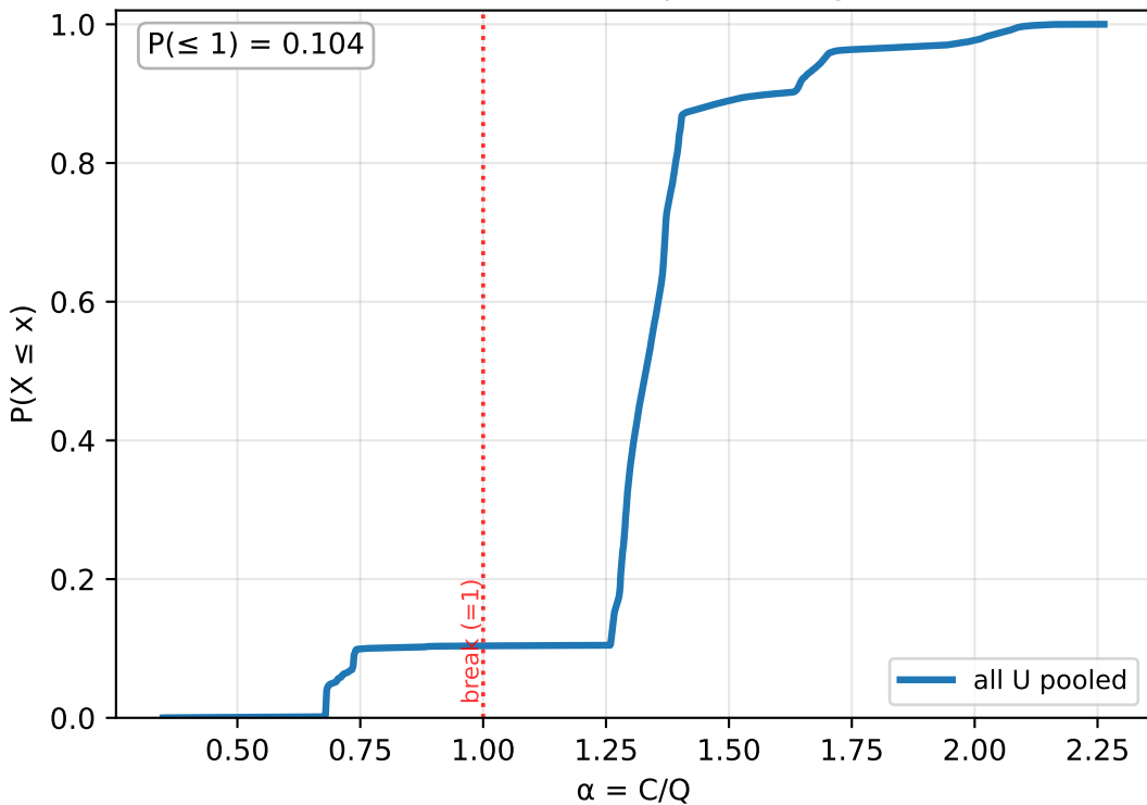
CDF of \alpha — all U pooled (tight)
