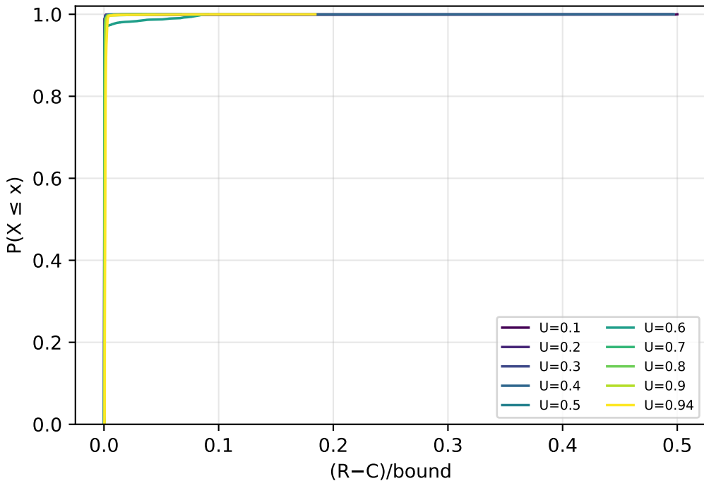
CDF of \Delta (soft)
