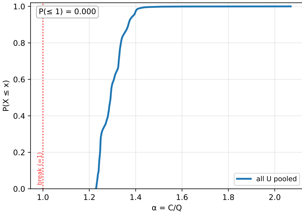
CDF of \alpha — all U pooled (soft)
