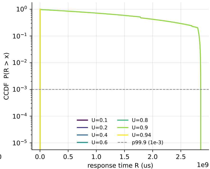
Model 1 — response-time tail (CCDF) [tb-20260708-1413-soft] tight (P = 10 ms) soft (P = 100 ms)
