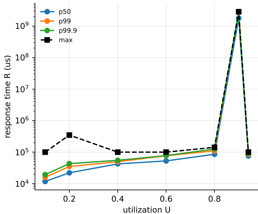
Model 1 — R percentiles vs U [tb-20260708-1413-soft]
