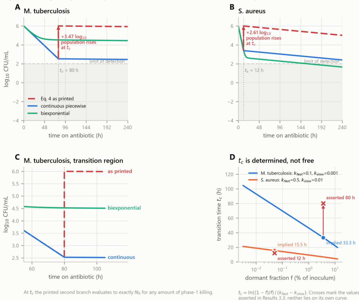
Figure 1. The closed-form biphasic law and its two corrections, all on the same parameters. (A, B) Equation 4a against the continuous piecewise and biexponential replacements. The arrow marks the upward jump at t_c : 3.47 log 10 for M. tuberculosis , 2.61 log 10 for S. aureus . (C) Detail of the transition region. At t_c the second branch of Equation 4a evaluates to exactly N_0 for any amount of first-phase killing. (D) The transition time is fixed by the other three parameters through Equation 4c. Crosses mark the values asserted in version 1; neither lies on its own curve.
