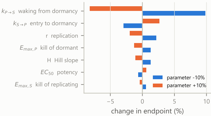
B the same OAT on the mechanistic model M. tuberculosis, time to sterilisation
