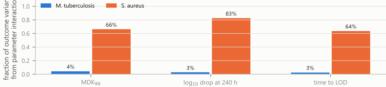
E what one-at-a-time analysis cannot see
