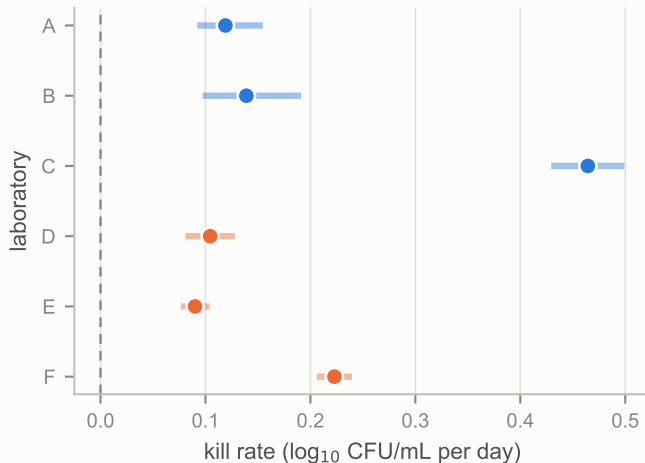
A A rate is estimable in all six
