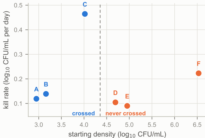
C The inoculum splits them; the rate does not
