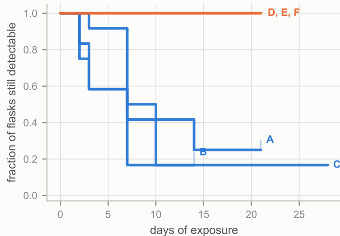
B A duration is undefined in three
