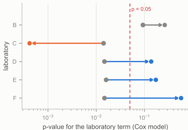
D Adjusting for the inoculum absorbs three of four
