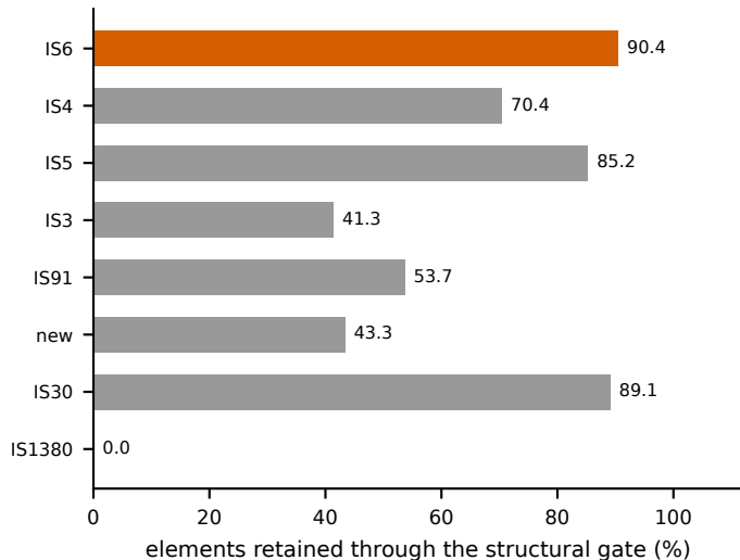
b IS6 is the best resolved abundant family
