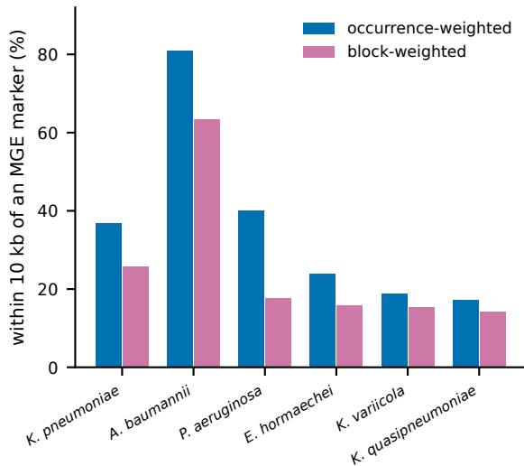
b Host ordering preserved
