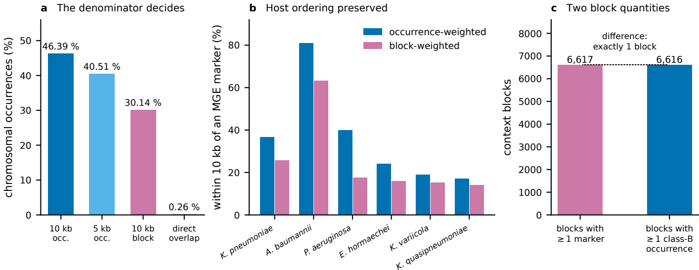
Figure 4 | 46.39 % of chromosomal occurrences lie within 10 kb of a mobile-element marker
