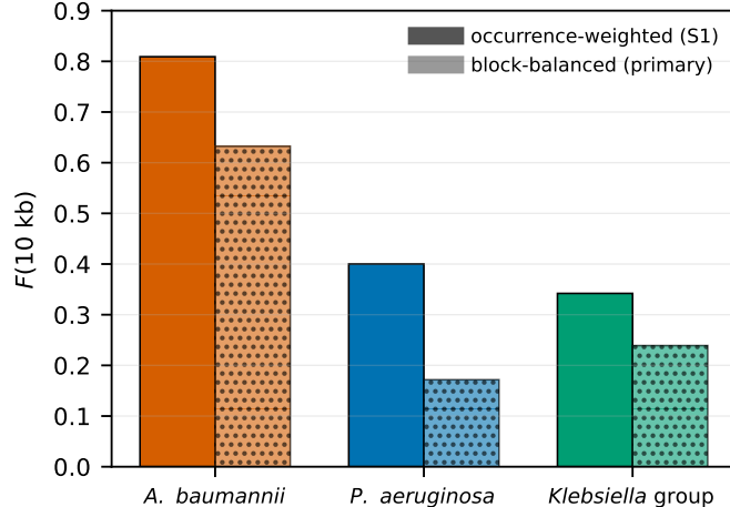
d Weighting sensitivity
