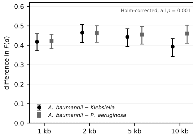
b Species contrasts at frozen landmarks
