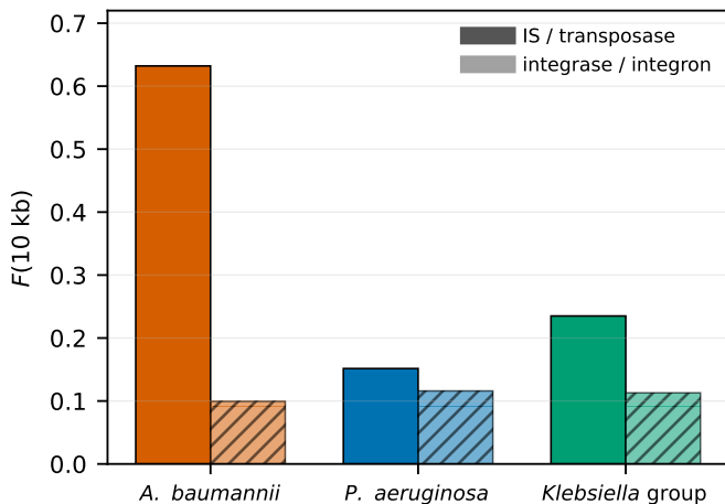
c Marker-type decomposition
