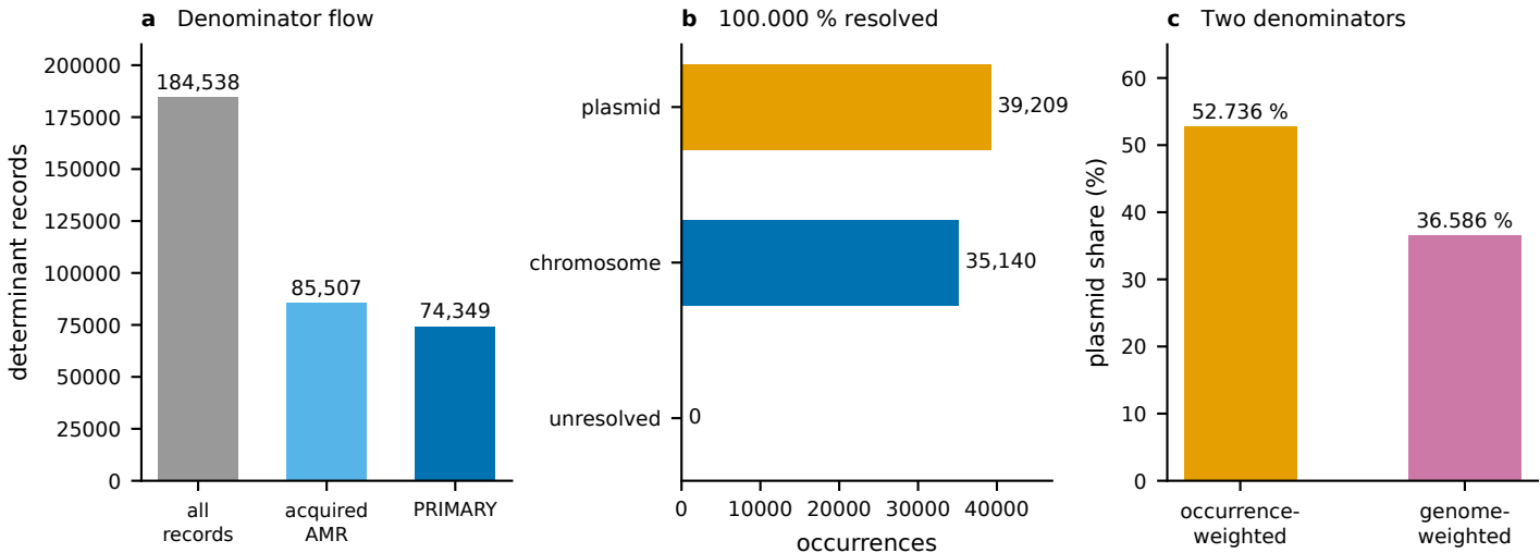
Figure 1 | 74,349 acquired resistance-gene occurrences in 6,288 closed genomes, each assigned to a documented replicon
