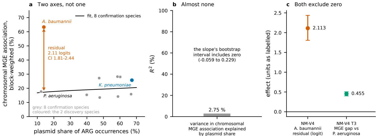
Figure 7 | Plasmid fraction and chromosomal mobile-element association are non-redundant, confirmed off the discovery species
