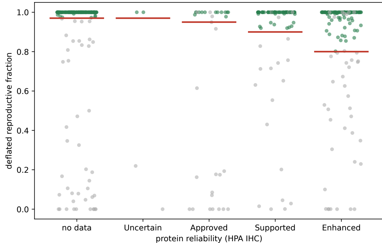
Protein reliability vs RNA fraction (HPA gate only) (red line = required RNA threshold for that tier)
