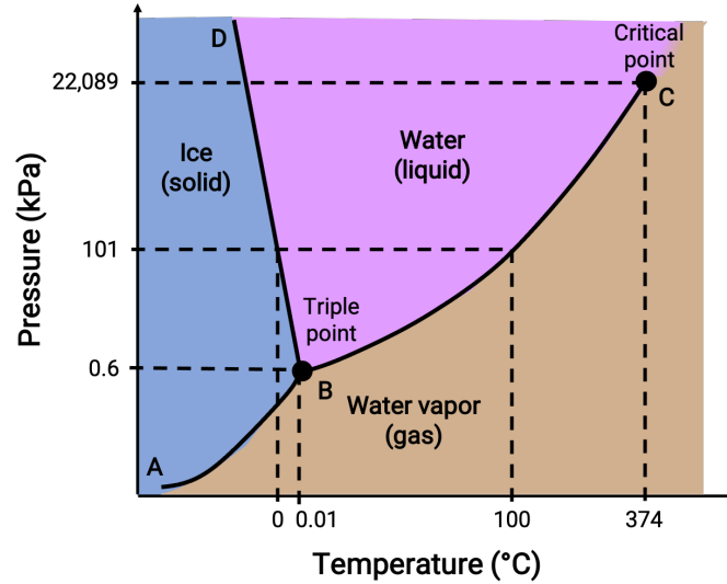
Fig. 12.1: The phase diagram of water.
