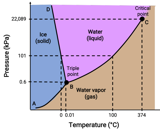
Fig. 5.1: The phase diagram of water.
