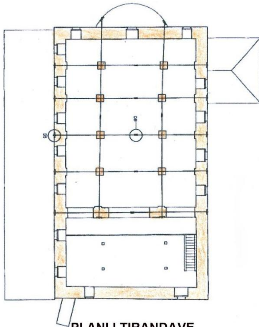
PLANI I TIRANDAVE
