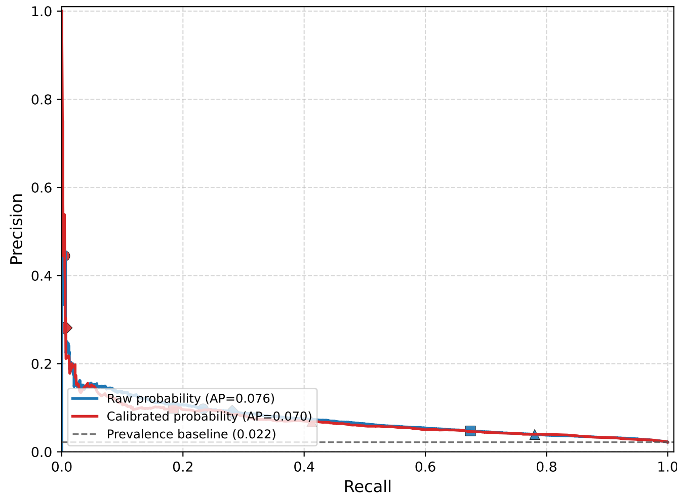
pretrain protocol
