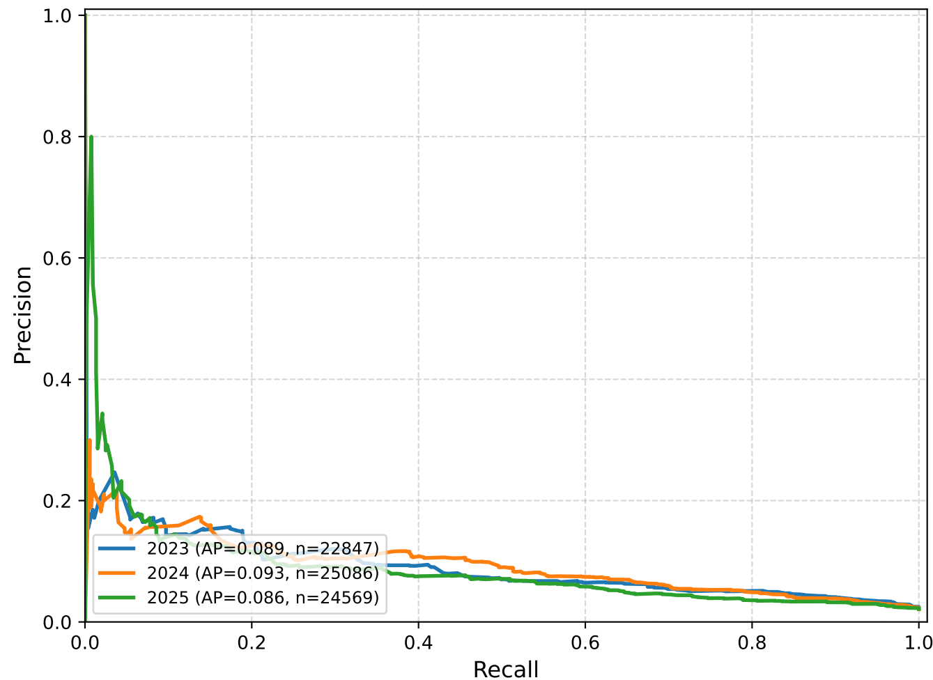
pretrain by year (calibrated)
