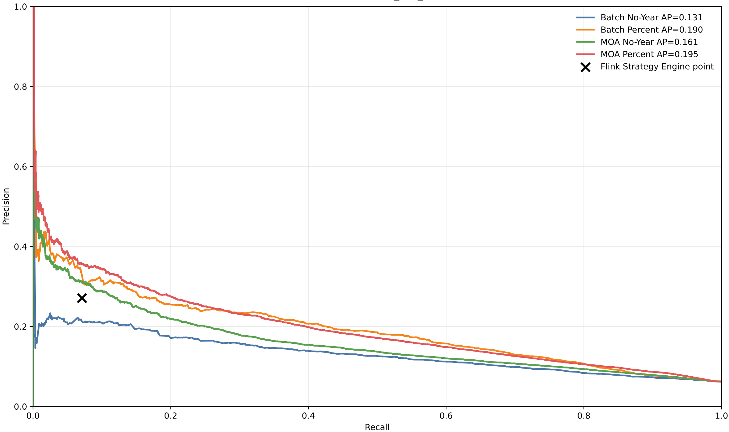
PR Curve — pit_any_h2
