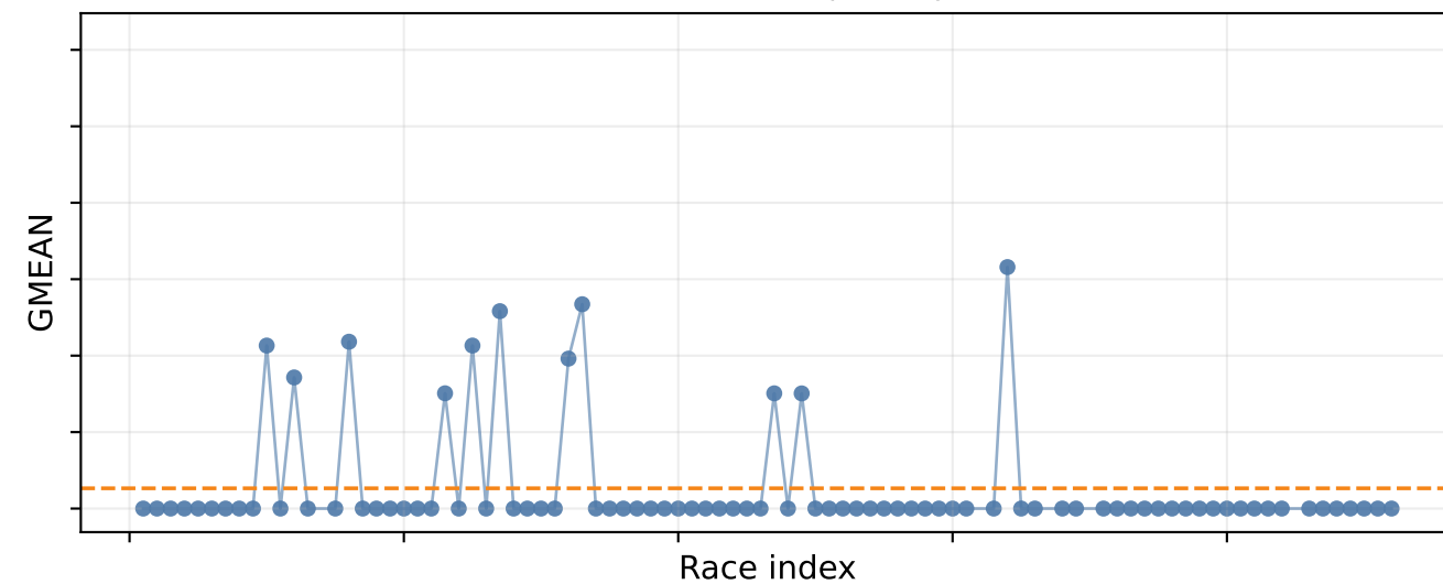
MOA No-Year (n=87)
