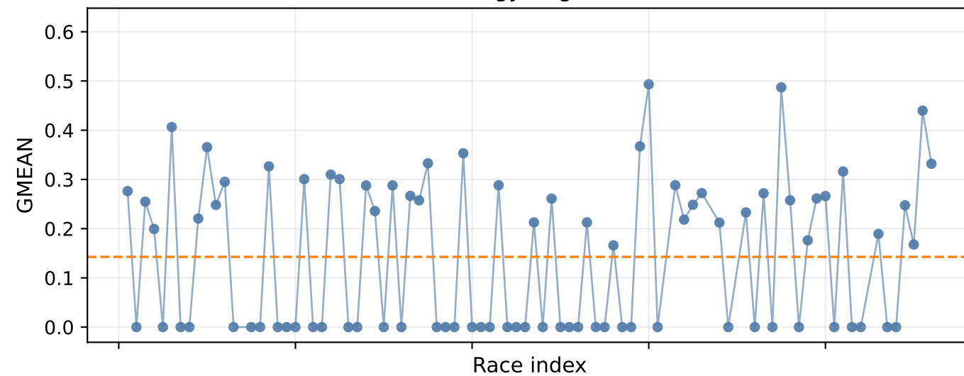
Batch Percent (n=86)
