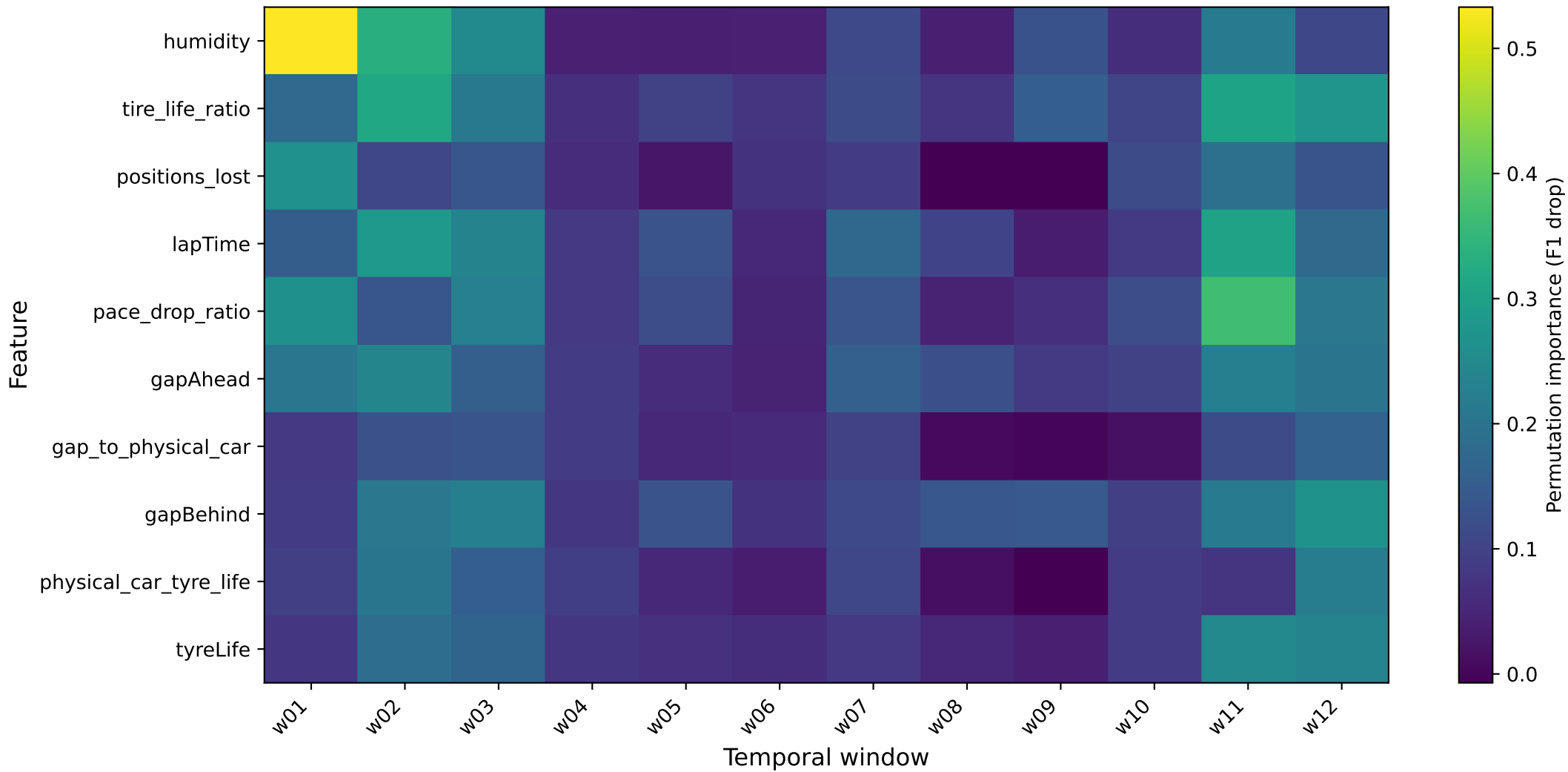
MOA Temporal Permutation Importance (F1 drop)
