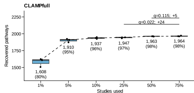
Supplementary Figure 4 | Complete pathway and trait coverage and saturation
