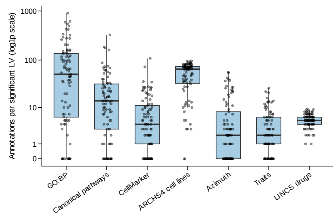
B Biological annotations of significant LVs
