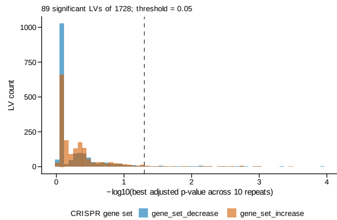
A CRISPR enrichment across all latent variables
