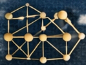
Context Modeling
