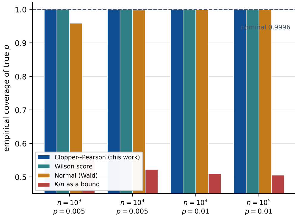
(a) coverage against a known ground truth
