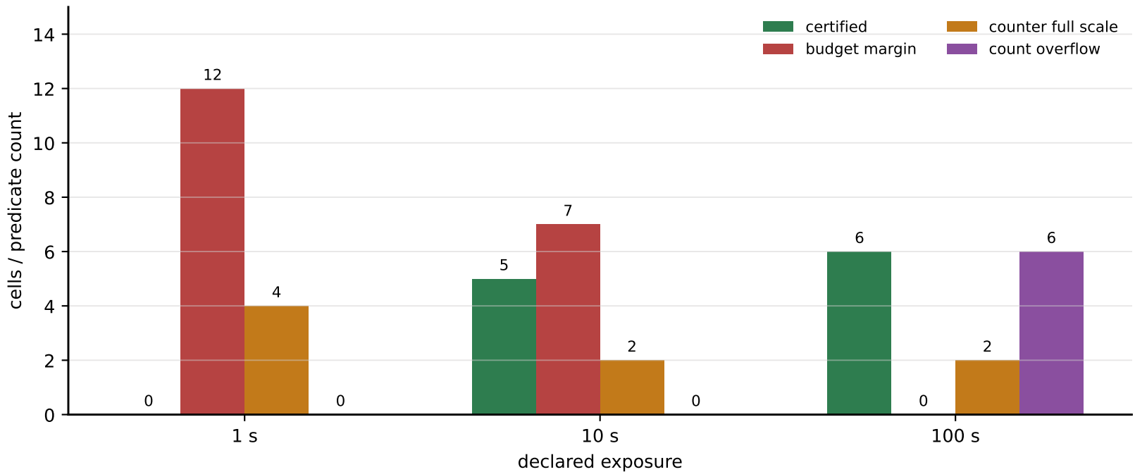
(a) Explicit-rate refusal predicates by exposure
