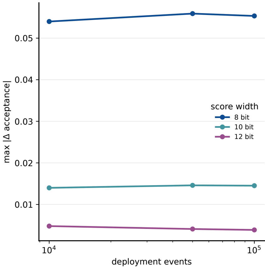
(a) score quantization audit
