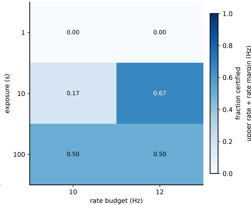
(b) certified fraction
