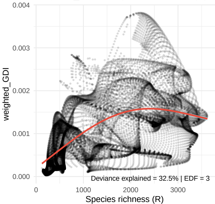
weighted_GDI vs. Species richness (R)
