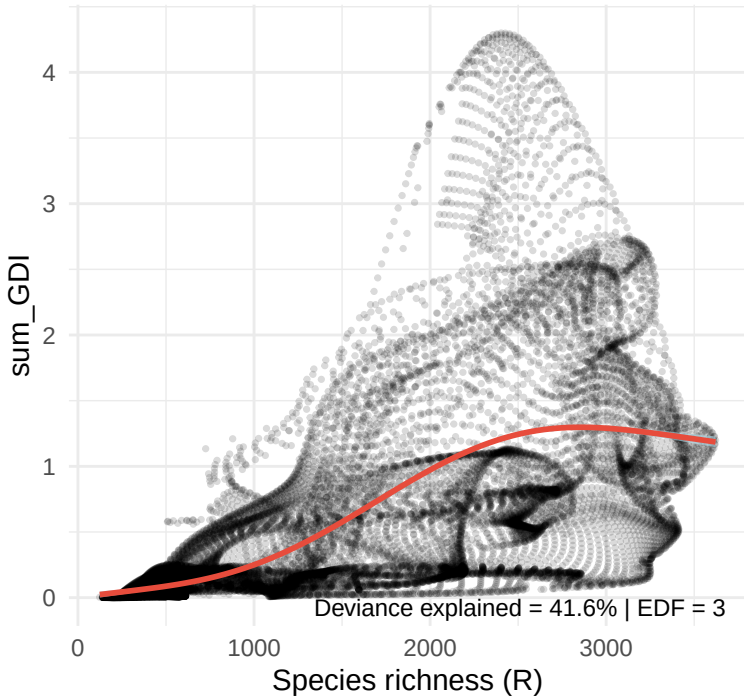
sum_GDI vs. Species richness (R)
