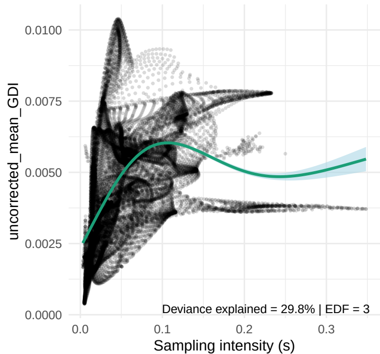
uncorrected_mean_GDI vs. Sampling intensity
