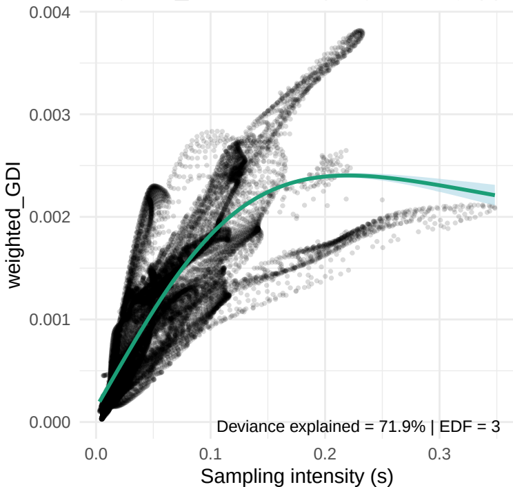
weighted_GDI vs. Sampling intensity (s)
