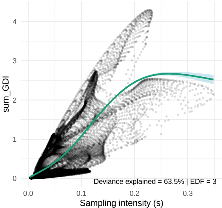
sum_GDI vs. Sampling intensity (s)
