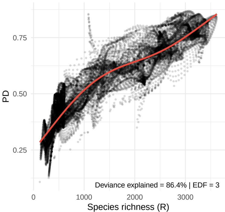
PD vs. Species richness (R)
