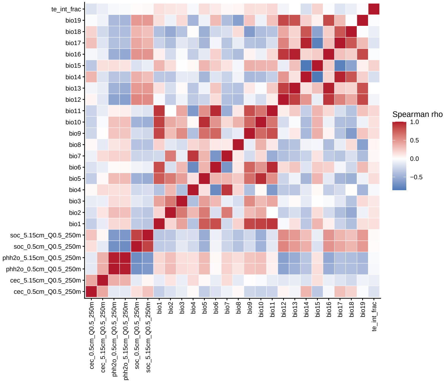
Environmental correlation matrix before filtering
