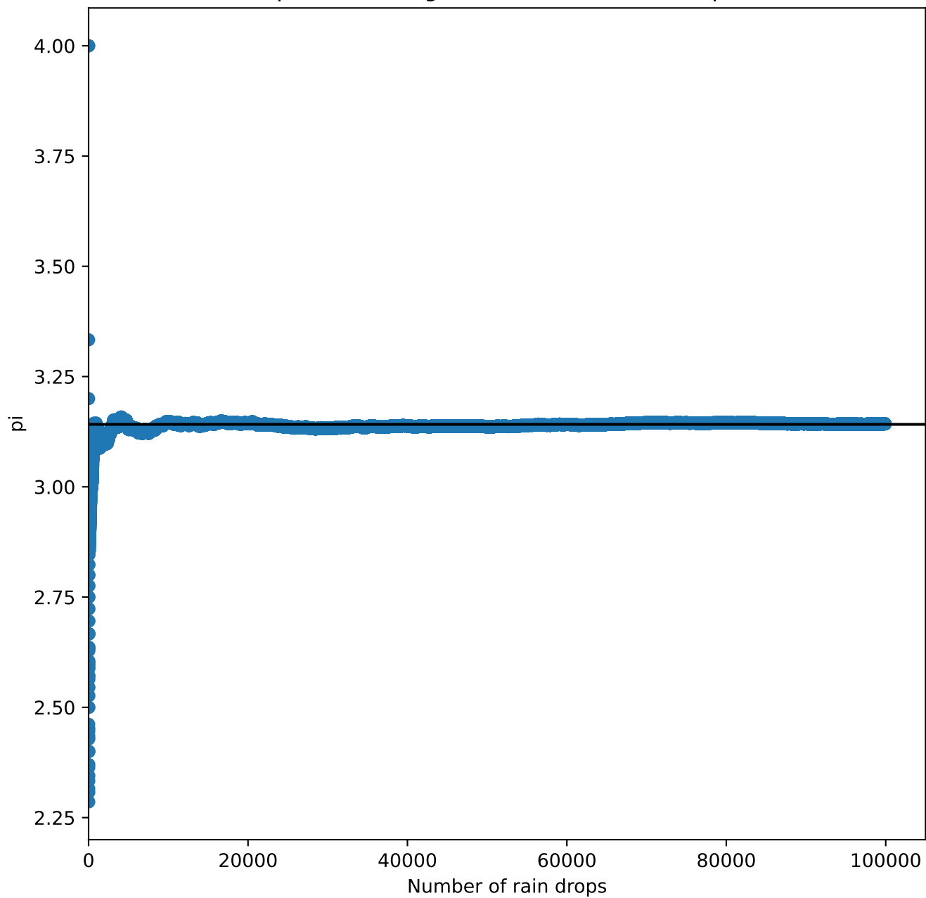
pi estimate against number of rain drops
