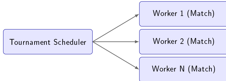
Figure 4.3. Parallel Worker Tournament Scheduler.
