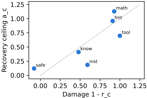
llama: damage vs recoverability
