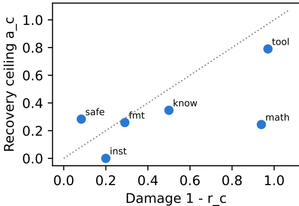
olmo: damage vs recoverability
