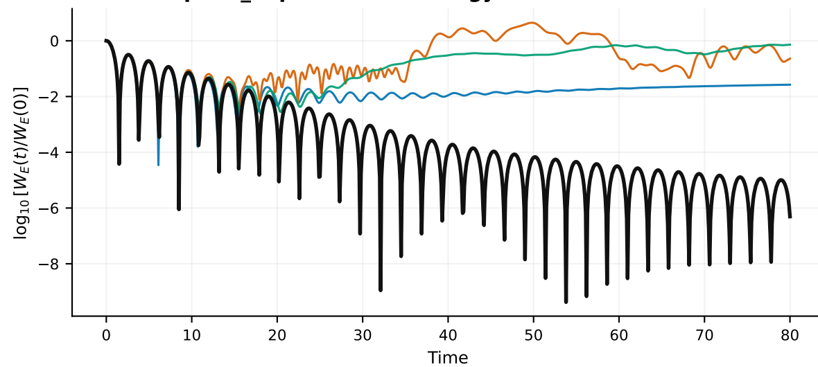
weak · K0p445_a0p030 · field energy
