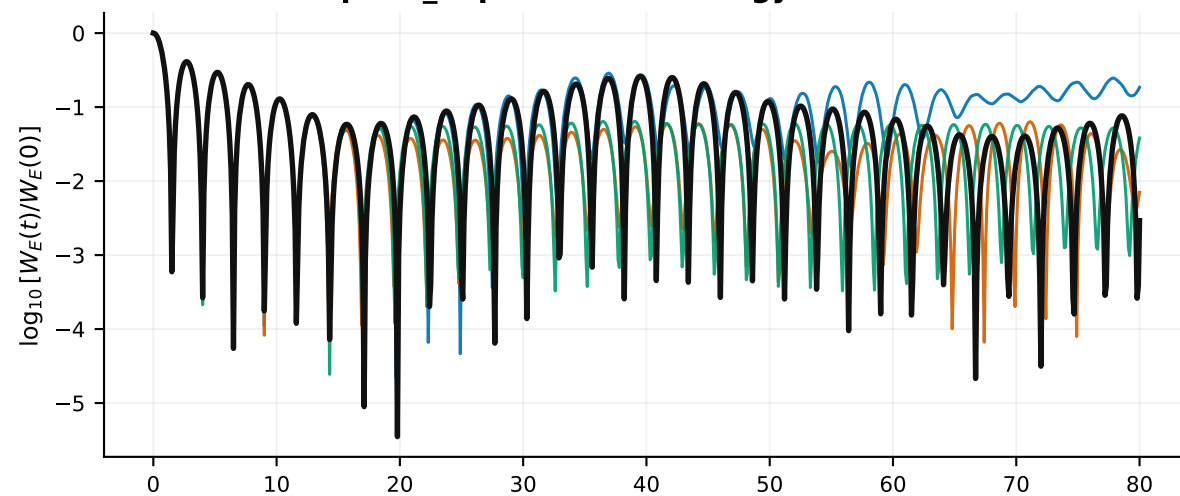
weak · K0p445_a0p030 · field energy
