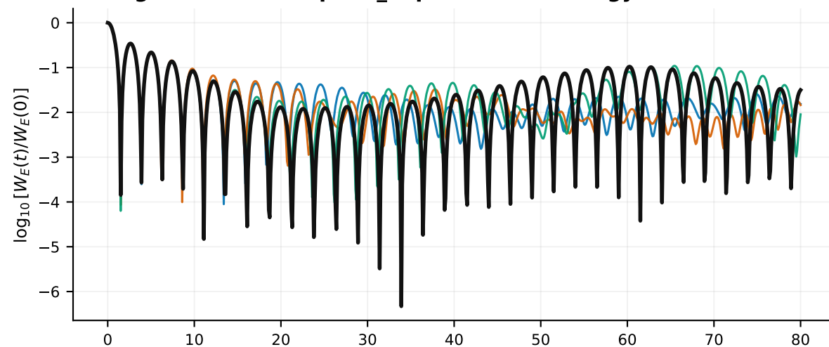
transition · K0p368_a0p186 · field energy
