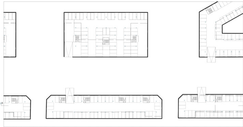
UNDERGROUND GARAGE 1:500
