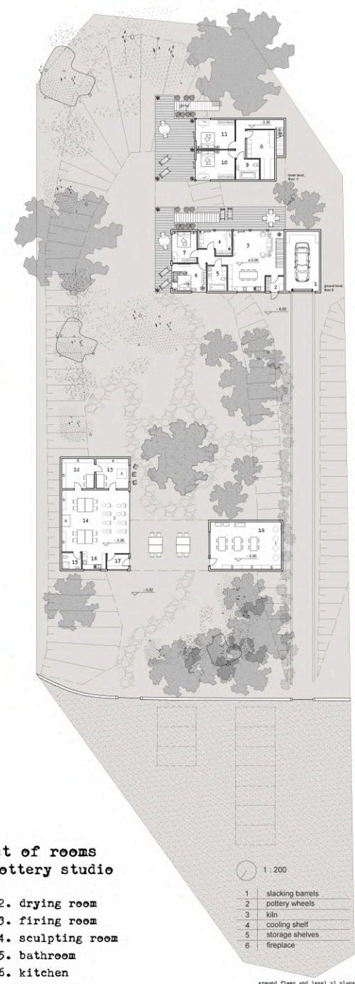
ground floor and level -1 plan
