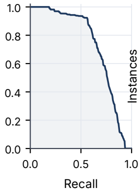
(c) Precision-recall
