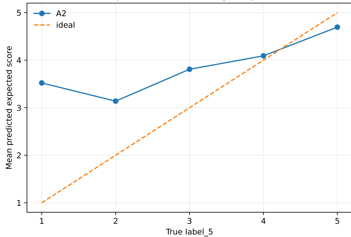
Exp3 Calibration Curve by Template
