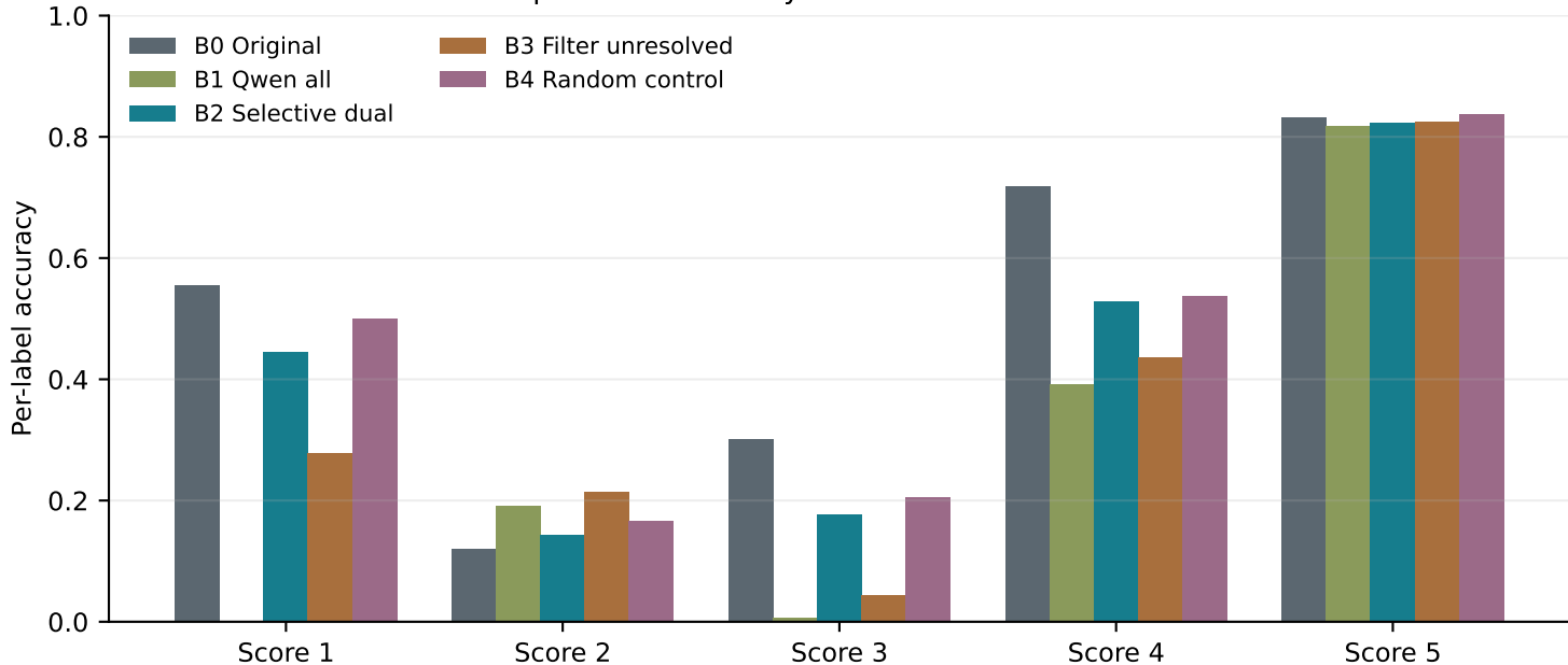
Exp28 Dev: accuracy across the full score scale
