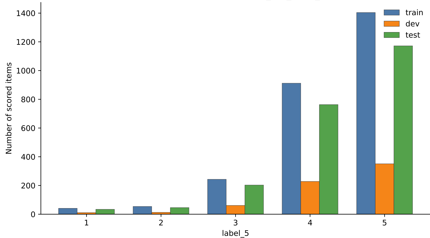
Label Distribution by Split (paper_like_triple_seed42)
