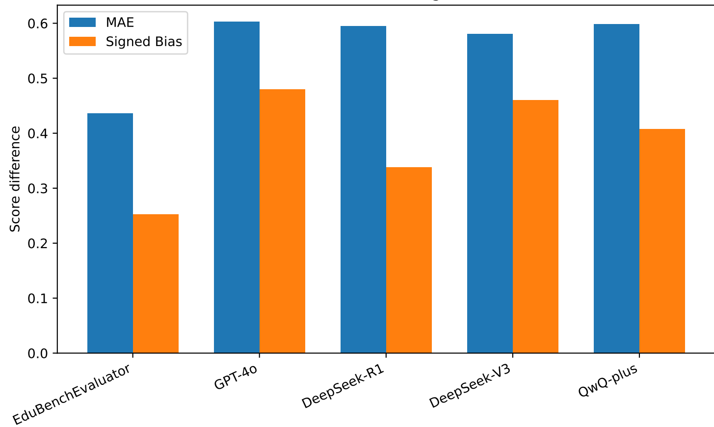
Evaluator MAE and Signed Bias
