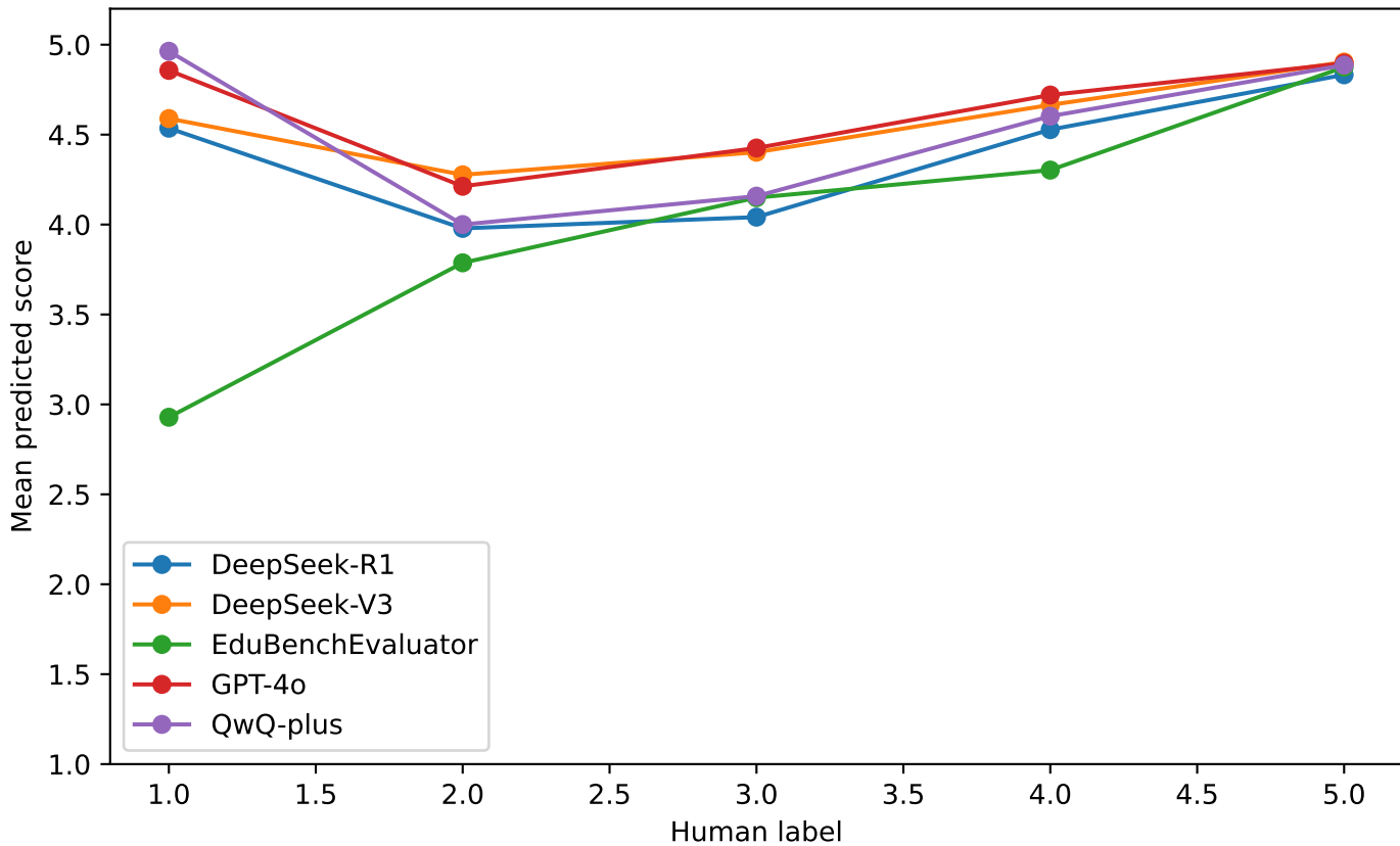
Mean Prediction by True Label
